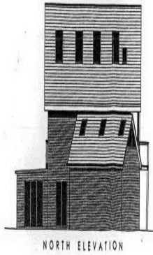
Proposed Elevations 06/3449/REV
